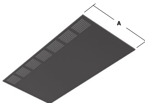
Vented soffit slotted to give 25mm continuous ventilation area
